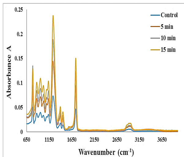
Fig.(9): FTIR spectrum of unexposed and exposure to different times of He-Ne laser of CR-39 nuclear track detector, at 10 mW laser power.
