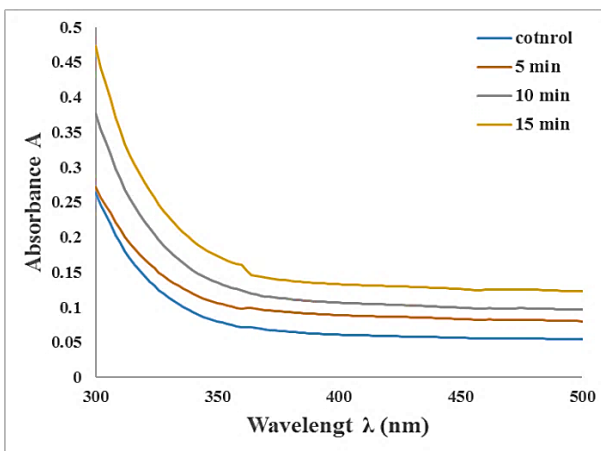
Fig.(5): UV-visible spectrum of CR-39 detector control and different exposure time of laser 5, 10, 15 min at power 5 mW, wavelength range from 300 nm to 500 nm.
