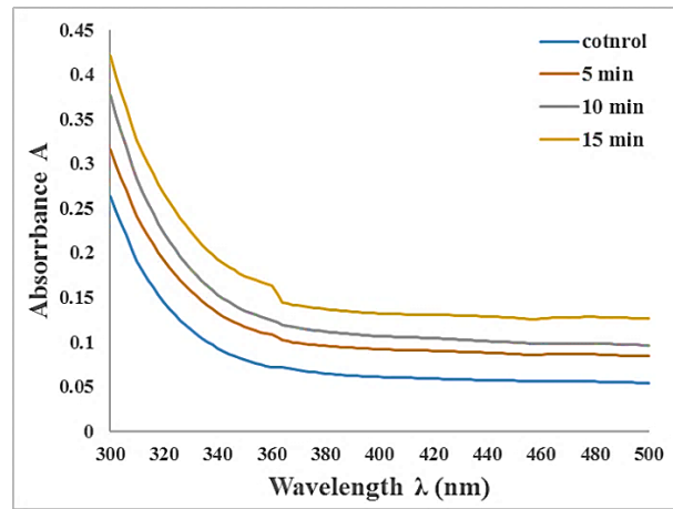
Fig.(6): UV-visible spectrum of CR-39 detector control with different exposure time of He-Ne laser 5, 10, 15 min at power 10 mW, wavelength range from 300 nm to 500 nm.
