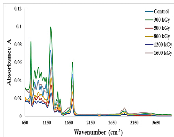
Fig.(10): FTIR spectrum of un-irradiated and irradiated of gamma ray of CR-39 nuclear track detector.
