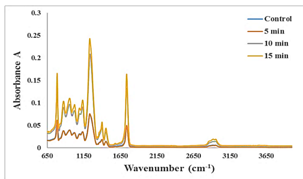
Fig.(8): FTIR spectrum of unexposed and exposure to different times of He-Ne laser of CR-39 nuclear track detector, at 5 mW laser power.
