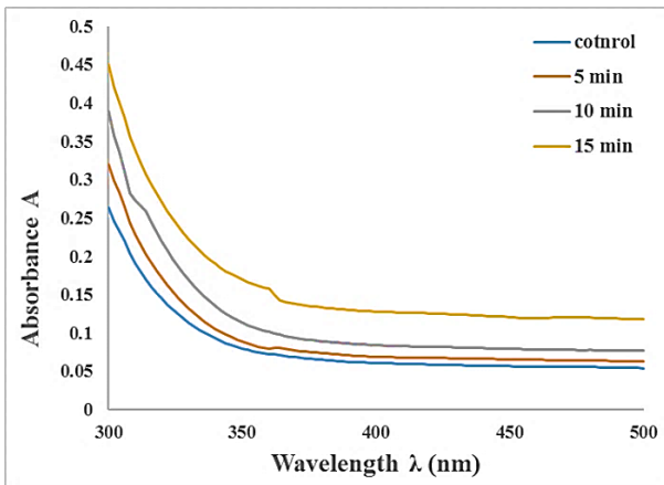
Fig.(4): UV-visible spectrum of CR-39 detector control and different exposure time of He-Ne laser 5, 10, 15 min at power 1 mW, wavelength range from 300 nm to 500 nm.
