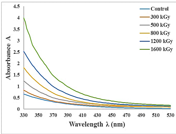
Fig.(3): UV-visible spectrum of CR-39 detector un-irradiated (control) and irradiated with gamma ray for doses 300, 500, 800, 1200 and 1600 kGy and exposed at 15 min of He-Ni laser of 10 mW power, wavelength range from 330 nm to 530 nm.
