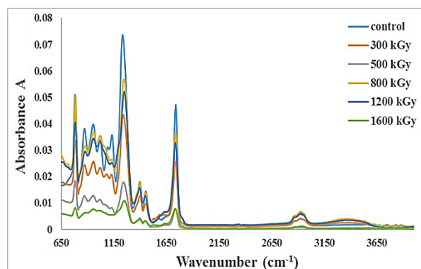
Fig.(11): FTIR spectrum of un-irradiated and irradiated of gamma ray of CR-39 nuclear track detector and exposed to He-Ne laser.
