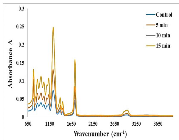
Fig.(7): FTIR spectrum of unexposed and exposure to different times of He-Ne laser of CR-39 nuclear track detector, at 1 mW laser power.
