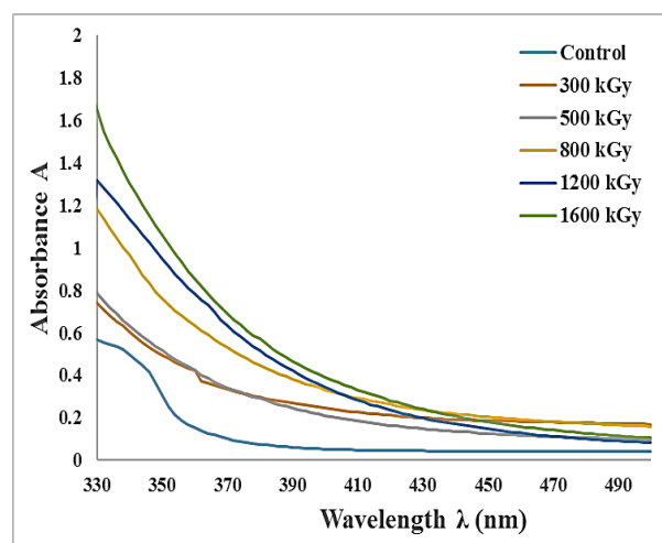
Fig.(2): UV-visible spectrum of CR-39 detector un-irradiated (control) and irradiated with gamma ray for doses 300, 500, 800, 1200 and 1600 kGy and wavelength range from 330 nm to 500 nm.
