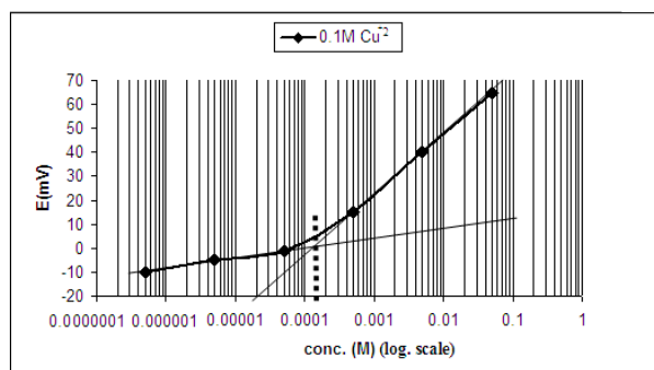
Fig.(4) Calibration curve of fixed interfering method using promethazine hydrochloride selective electrode using DBPH plasticizer.
