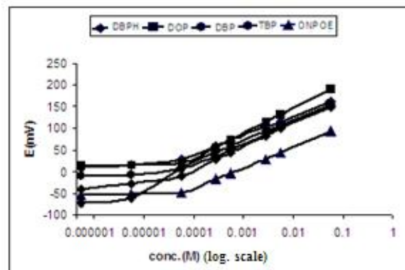
Fig.(2) Calibration curves of promethazine hydrochloride selective electrodes using DPB, DBPH, DOP, TBP and ONPOE plasticizers.
