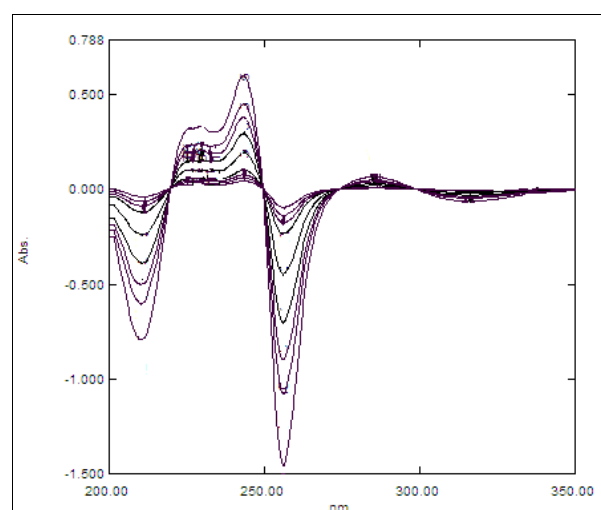
Fig.(8) The first derivative spectra for Promethazine hydrochloride solutions at different concentration ranged from 2 to 62 mg/L.
