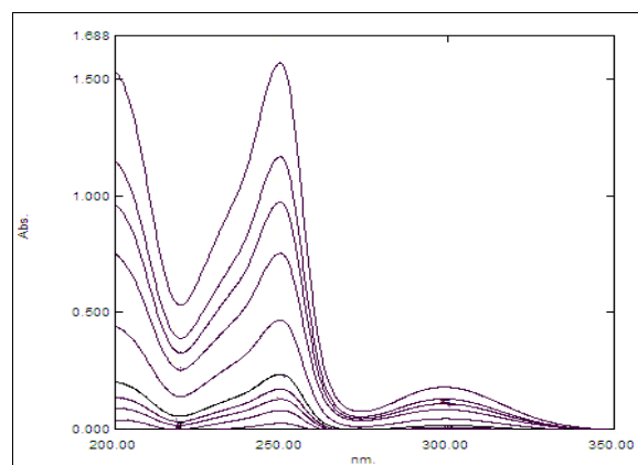
Fig.(7) Spectra for Promethazine hydrochloride solutions at different concentration ranged from 2 to 62 mg/L.
