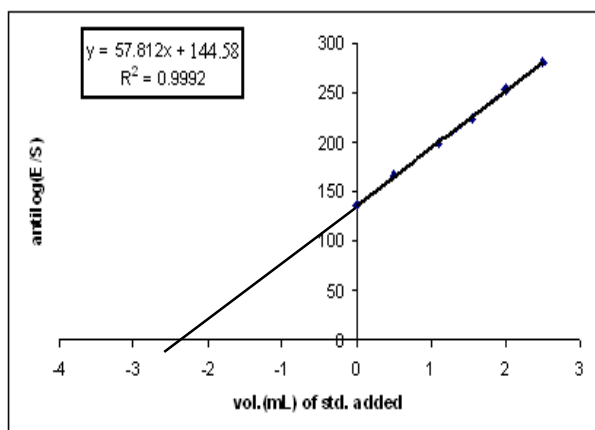
Fig.(5) Plot of antilog (E/S) versus the volume of promethazine using metode using promethazine hydrochloride selective electrode using DBPH plasticizer.
