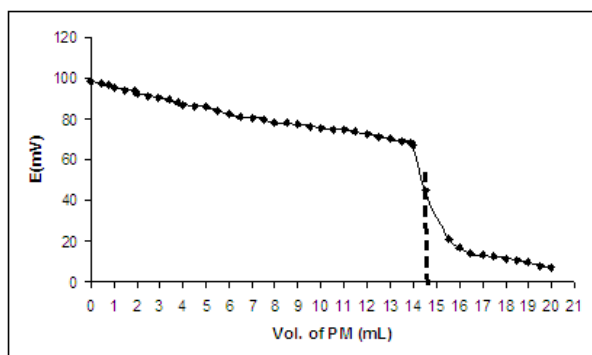
Fig.(6) Titration curve of promethazine hydrochloride selective electrode using DBPH plasticizer.
