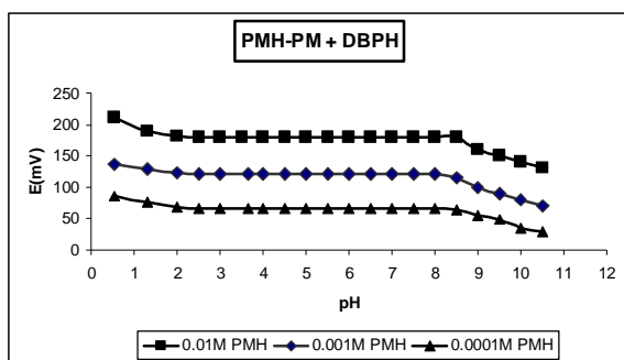
Fig.(3) Effect of pH on the potential of promethazine hydrochloride selective electrode using DBPH plasticizer.
